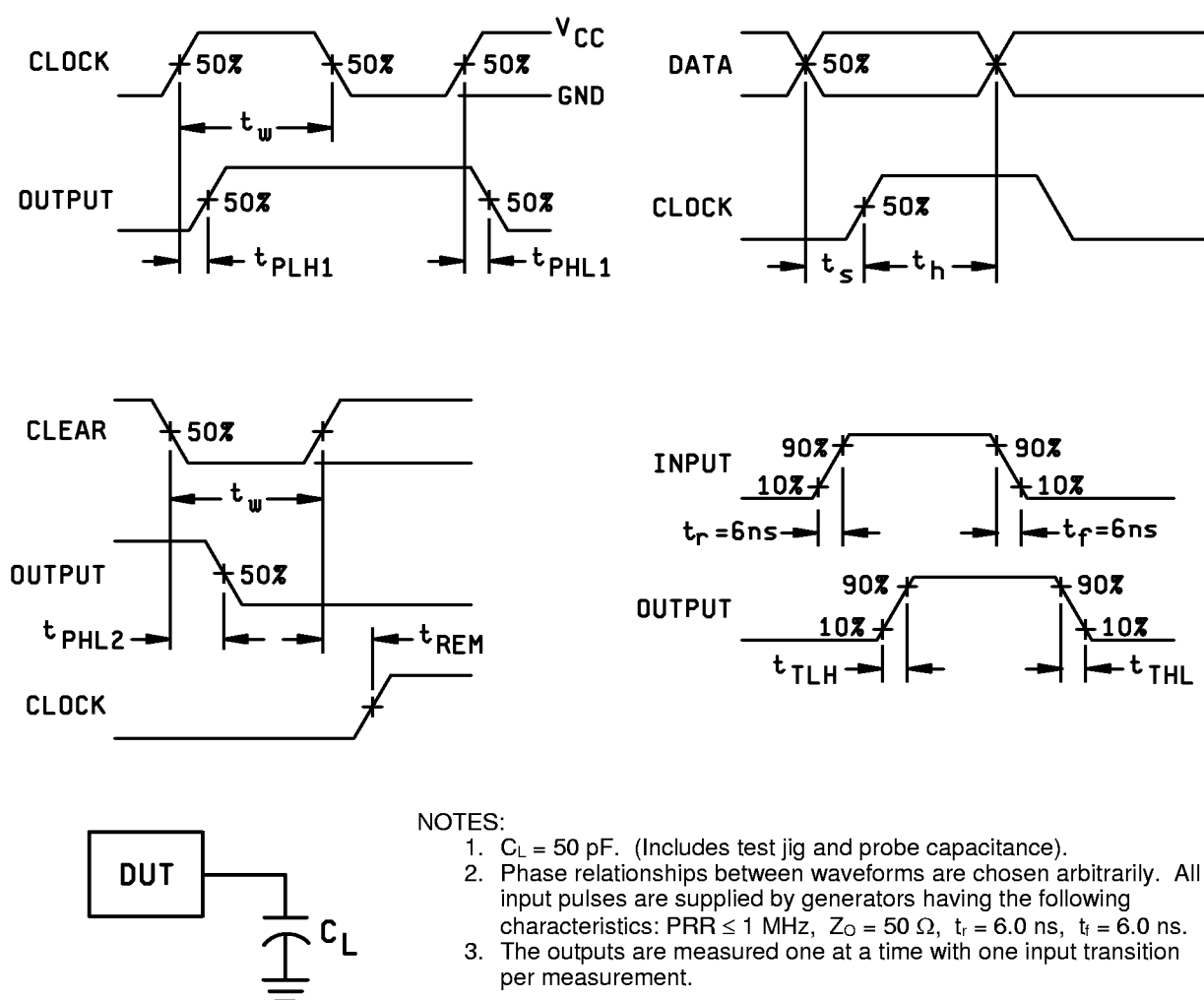
FIGURE 4. Switching waveforms and test circuit.
