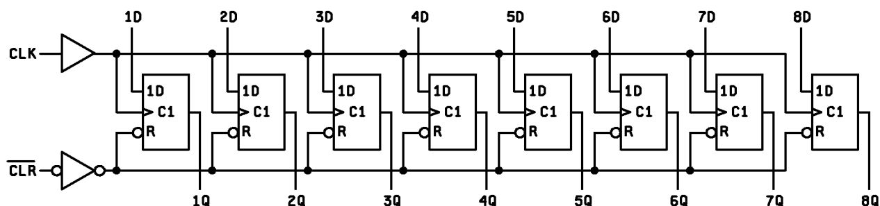
FIGURE 3. Logic diagram.
