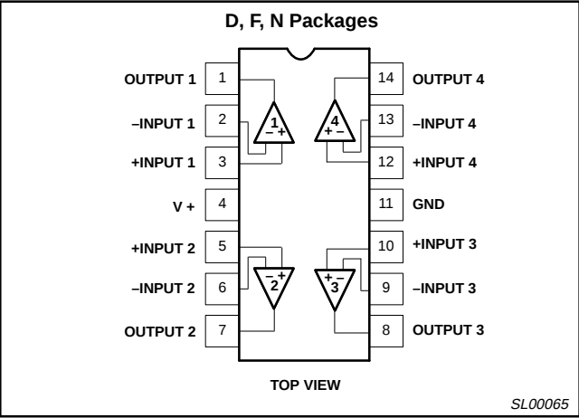
Figure 1. Pin Configuration
