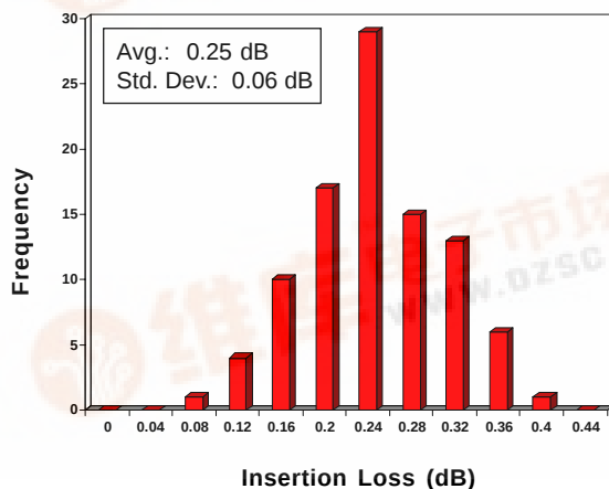
Insertion Loss Performance (SM, APC ferrule, 9/125 \mu m fiber)
