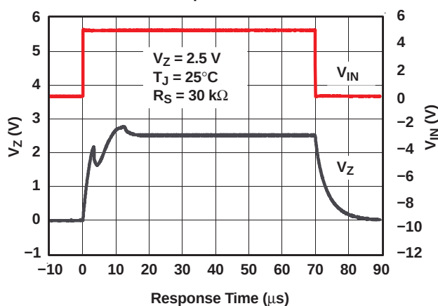
Figure 6. Start-Up Characteristics
