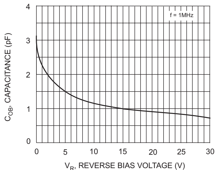
Fig. 4 Output Capacitance
