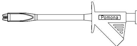
MODEL 5912B MAXIGRABBER TEST CLIP SET WITH JAWS QTY 2 : 1 RED, 1 BLACK
