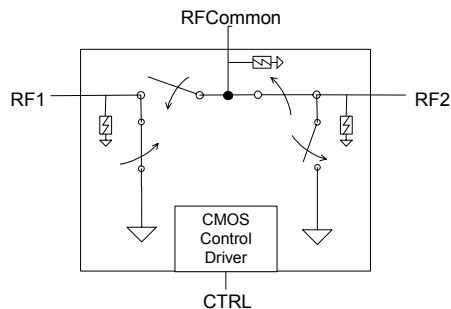
Figure 1. Functional Diagram
