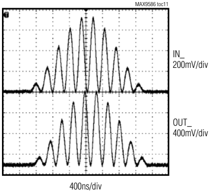
12.5T RESPONSE
