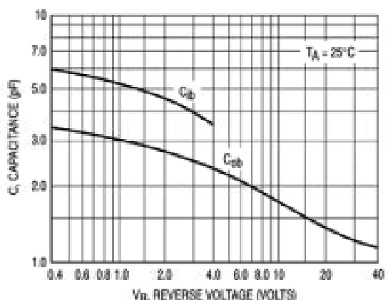
Figure 5. Capacitances
