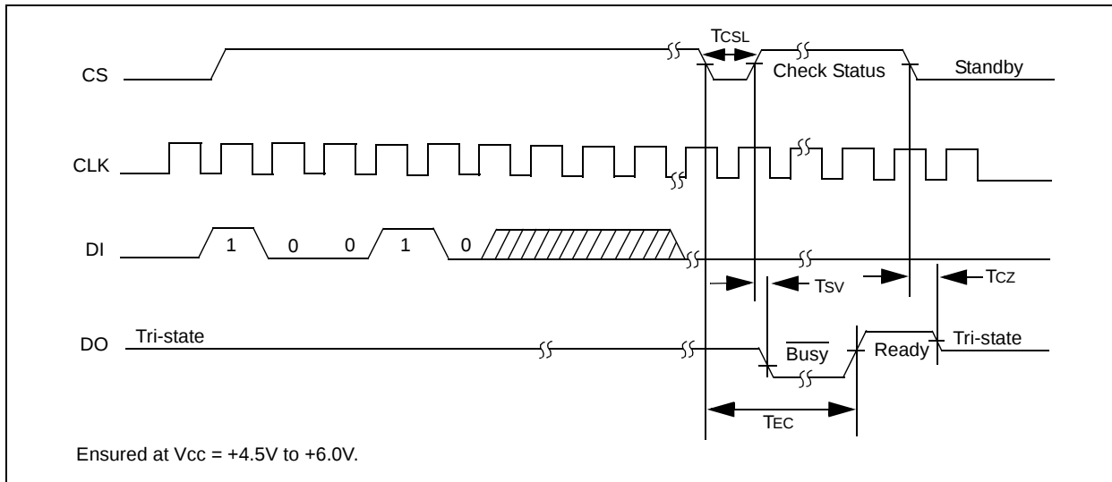
FIGURE 2-8: SERIAL TIMING
