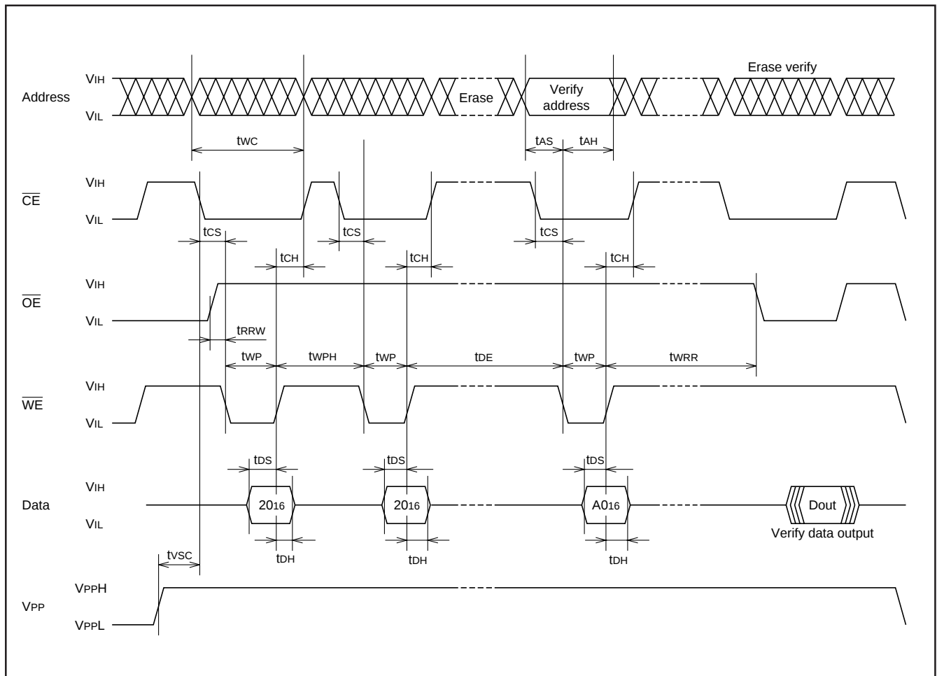
Fig. 70 Input/output timings during erasing (verify data is output at the same timing as for read.)
