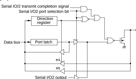
(24) Port P73
