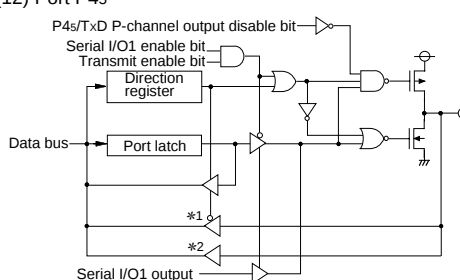
(12) Port P45
