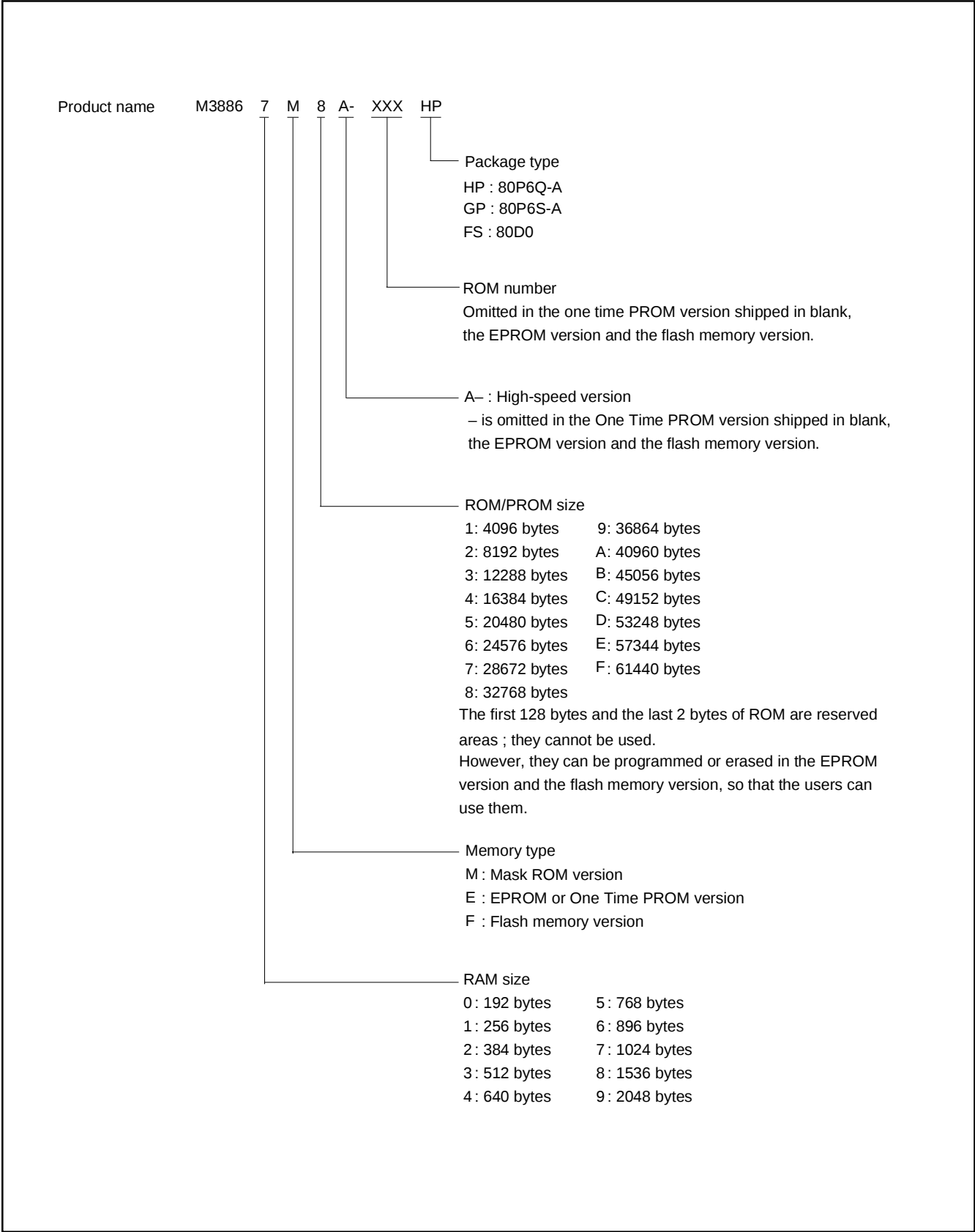
Fig. 5 Part numbering
