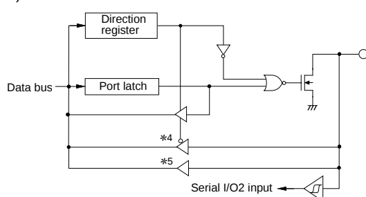
(21) Port P70
