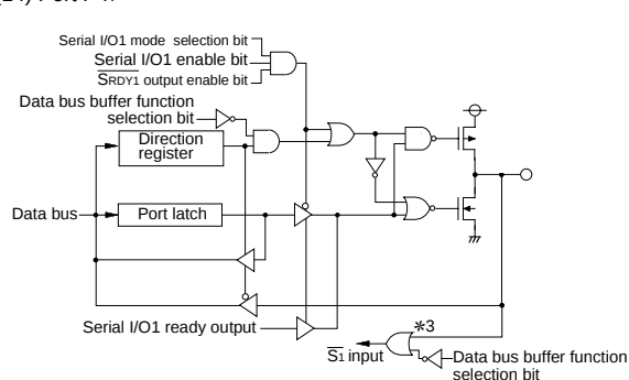
(14) Port P47
