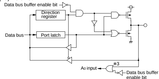
(15) Port P50
