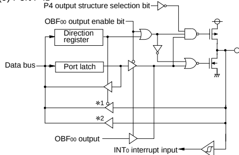
(9) Port P42
