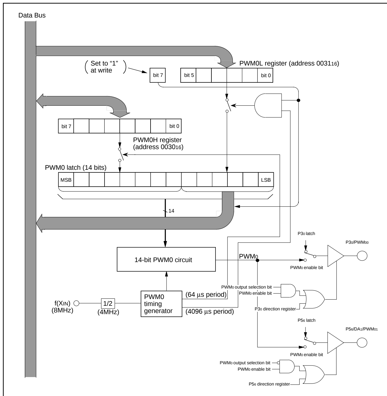
Fig. 29 PWM block diagram (PWM0)
