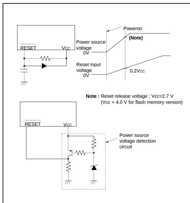
Fig. 55 Reset circuit example
