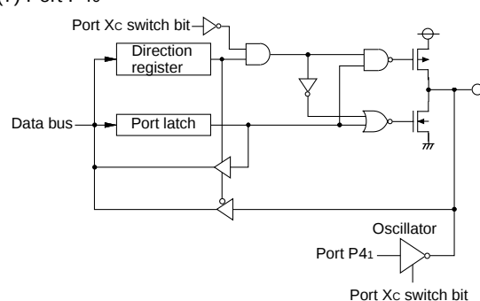
(7) Port P40
