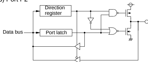
(3) Port P2
