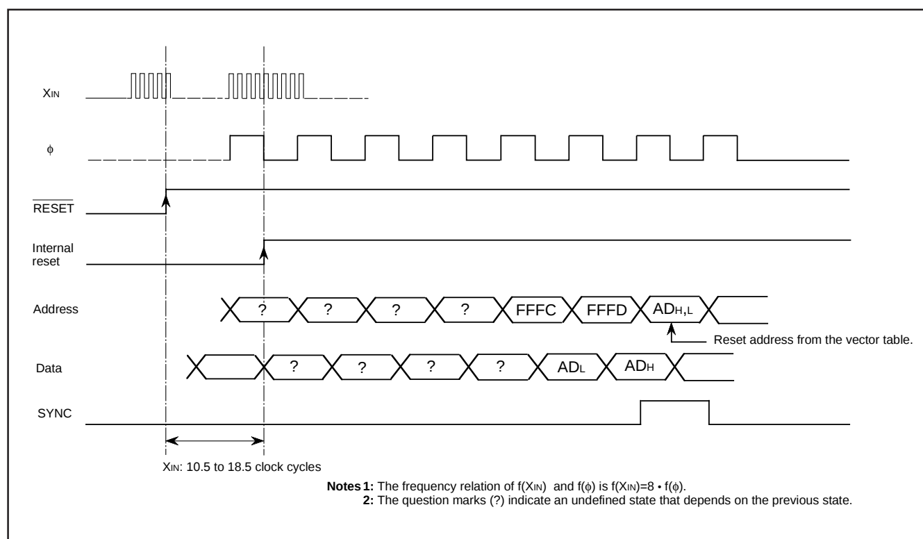
Fig. 56 Reset sequence
