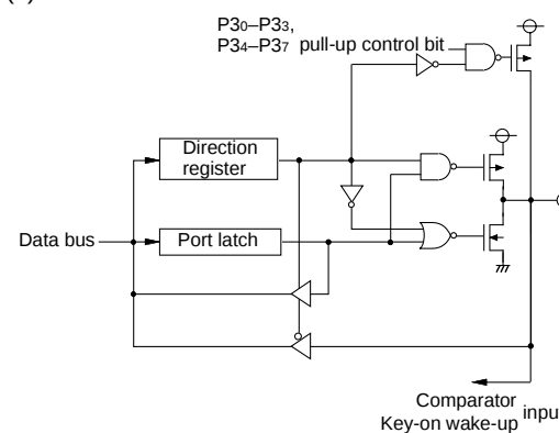
(6) Ports P32–P37
