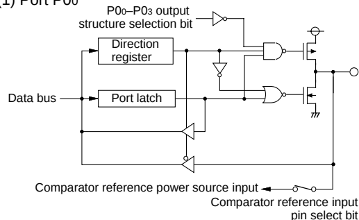
(1) Port P00
