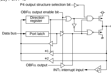
(10) Port P43
