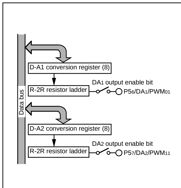
Fig. 50 Block diagram of D-A converter
