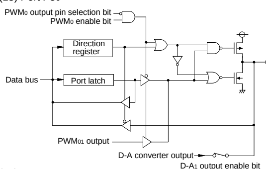
(20) Port P6
