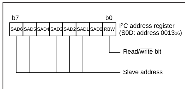
Fig. 36 Structure of I 2 C address register
