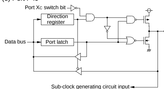
(8) Port P41
