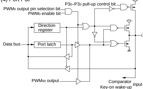
(4) Port P30
