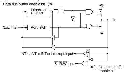
(16) Ports P51,P52,P53
