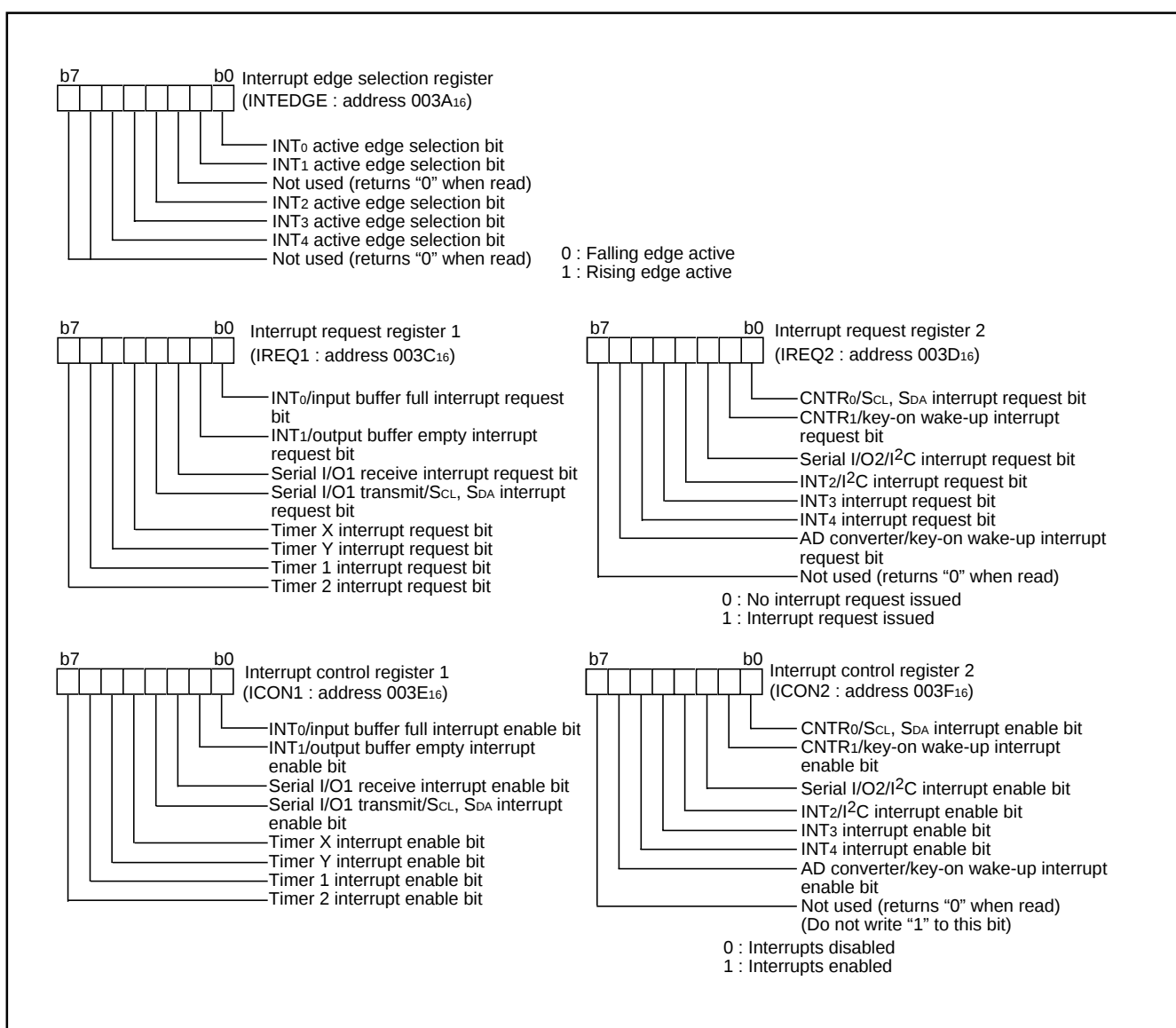
Fig. 16 Structure of interrupt-related registers (1)
