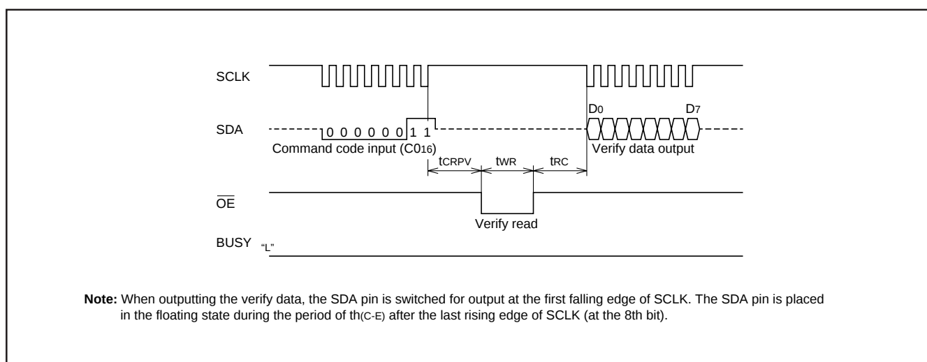
Fig. 75 Timings during program verify
