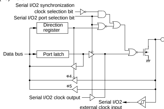
(23) Port P72
