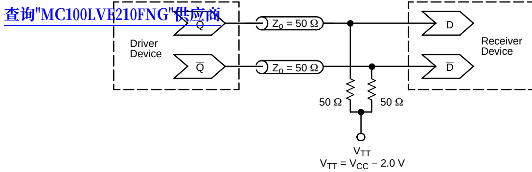
Figure 3. Typical Termination for Output Driver and Device Evaluation (See Application Note AND8020/D – Termination of ECL Logic Devices.)
