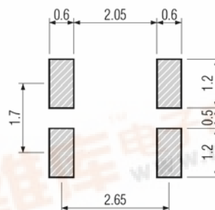
Figure 2) Suggested Land Pattern
