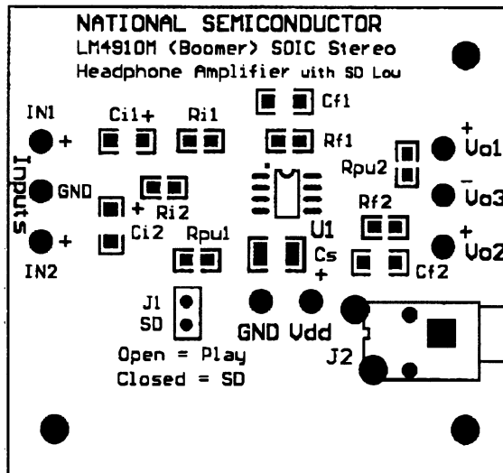
Silk Screen
