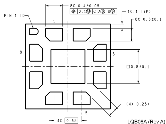
LQ Order Number LM4910LQ NS Package Number LQB08A
