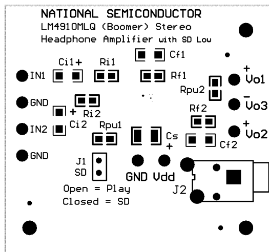
Silk Screen
