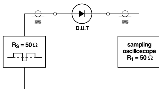
Test circuit
