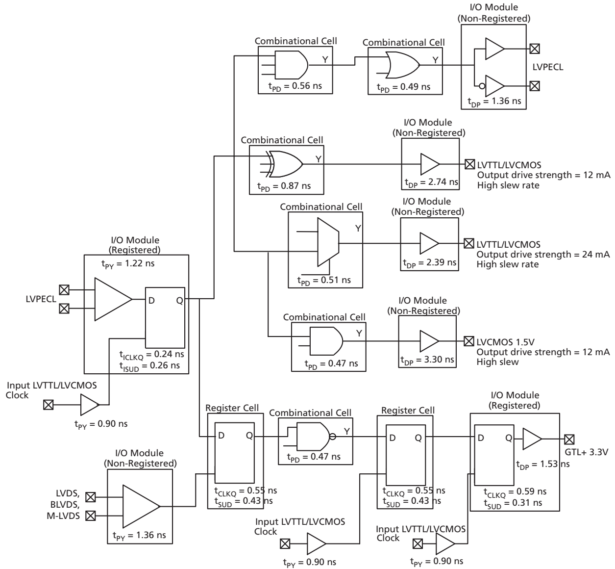
Figure 2-2 • Timing Model
