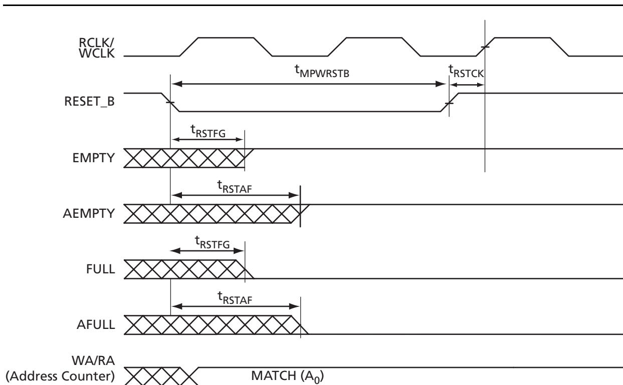
Figure 2-49 • FIFO Reset
