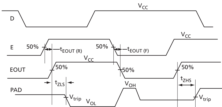
Figure 2-5 • Tristate Output Buffer Timing Model and Delays (example)
