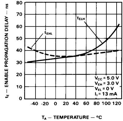
Figure 9. Enable Propagation Delay vs. Temperature.
