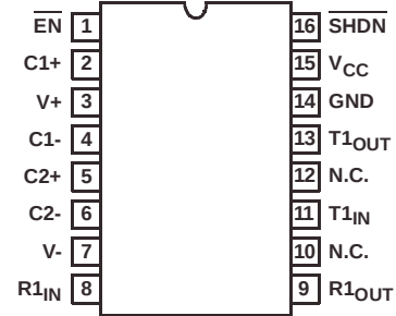
ISL83220E (SOIC, SSOP, TSSOP) TOP VIEW
