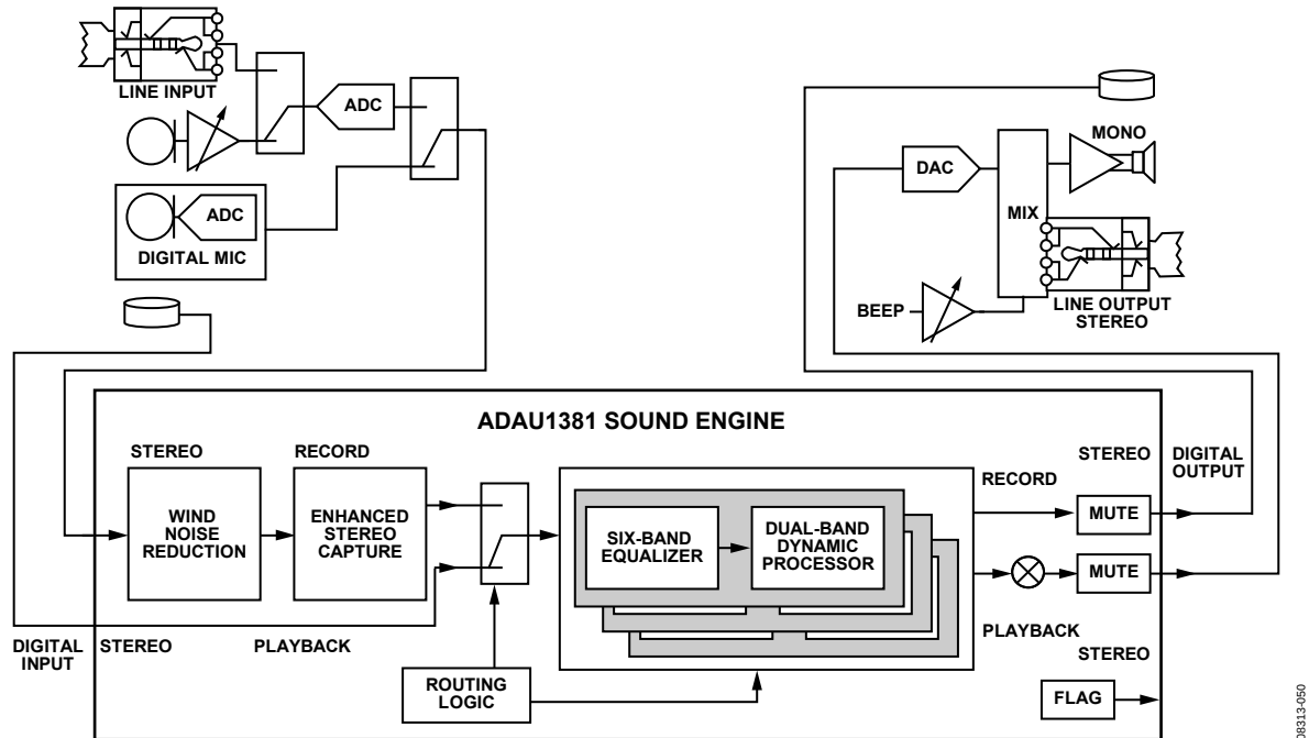
Figure 52. Sound Engine Signal Processing Flow
