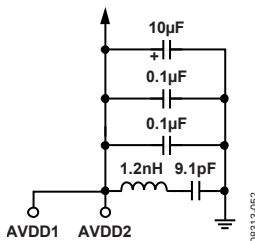
Figure 54. GSM Filter on the Analog Supply Pins
