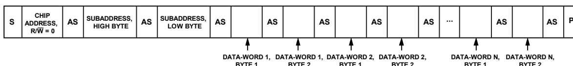
Figure 41. Burst Mode I 2 C Write Sequence
