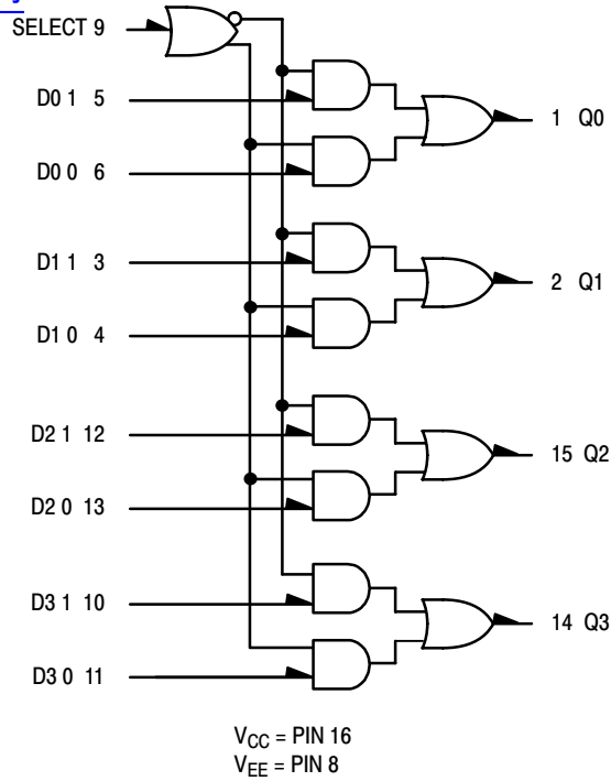
LOGIC DIAGRAM
