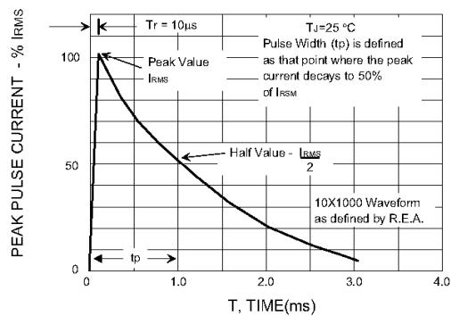
FIG.5 - PULSE WAVEFORM
