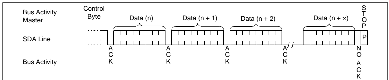
FIGURE 8-3: SEQUENTIAL READ
