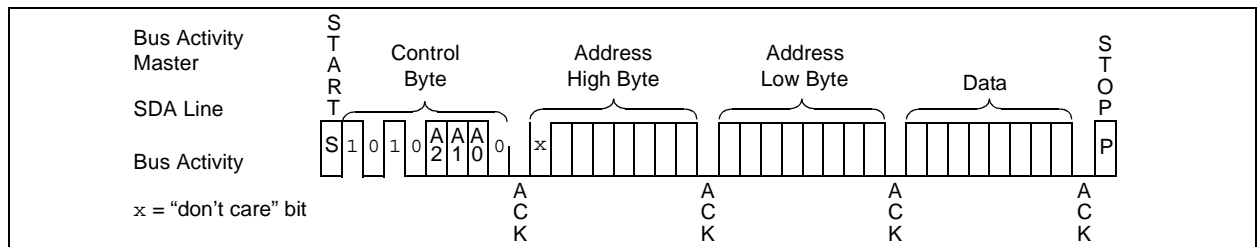
FIGURE 6-2: PAGE WRITE
