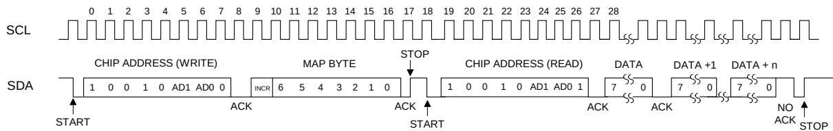
Figure 18. Control Port Timing, I²C Read
