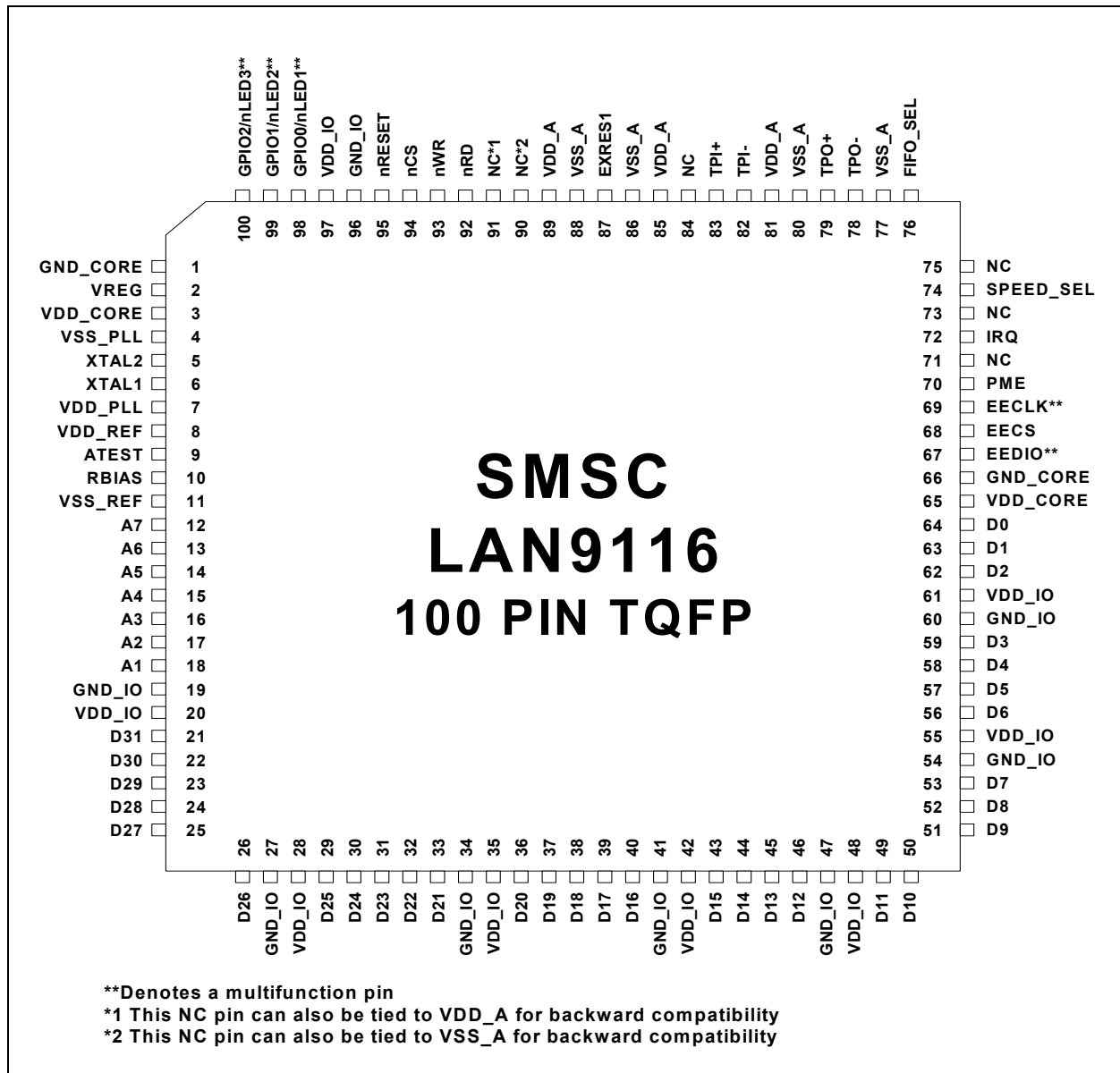
Figure 2.1 Pin Configuration
