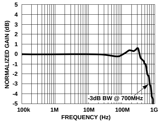
FIGURE 2. -3dB BANDWIDTH
