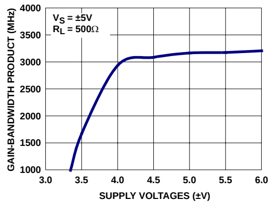
FIGURE 6. GAIN BANDWIDTH PRODUCT vs SUPPLY VOLTAGES
