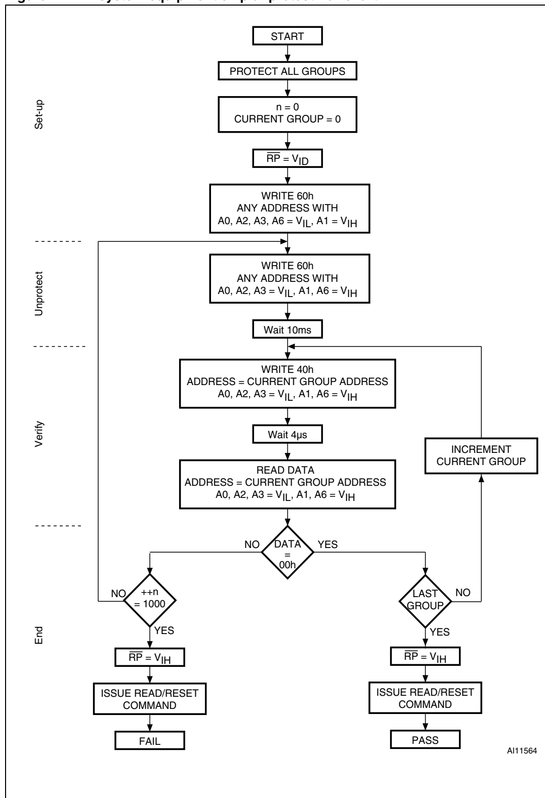
Figure 17. In-system equipment chip unprotect flowchart
