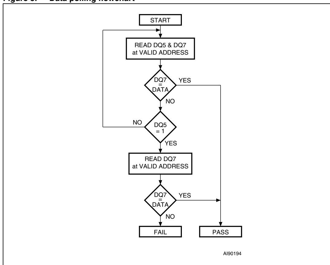
Figure 3. Data polling flowchart
