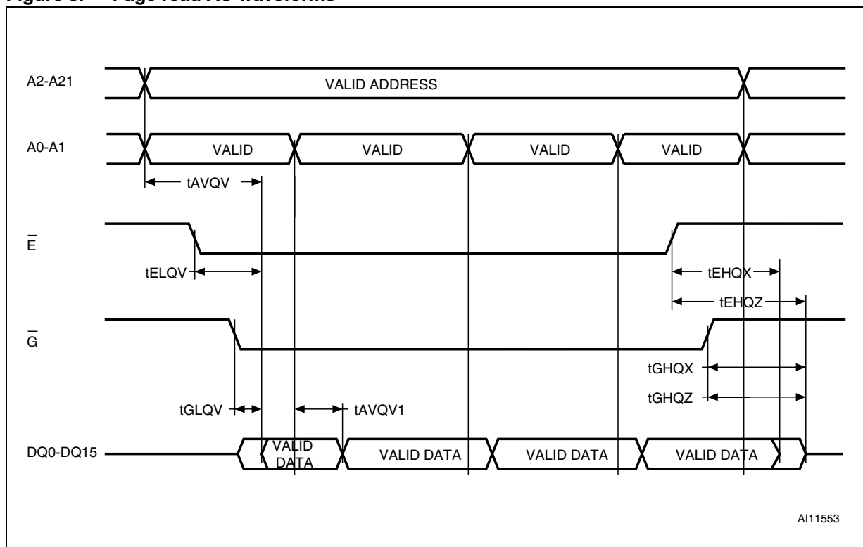
Figure 8. Page read AC waveforms
