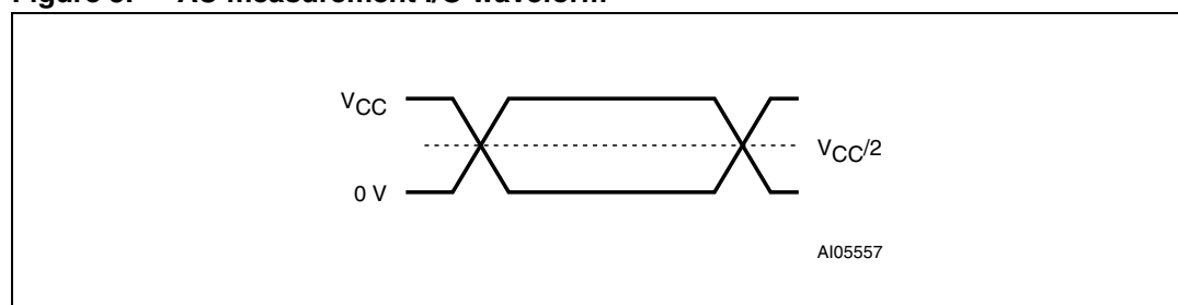
Figure 5. AC measurement I/O waveform
