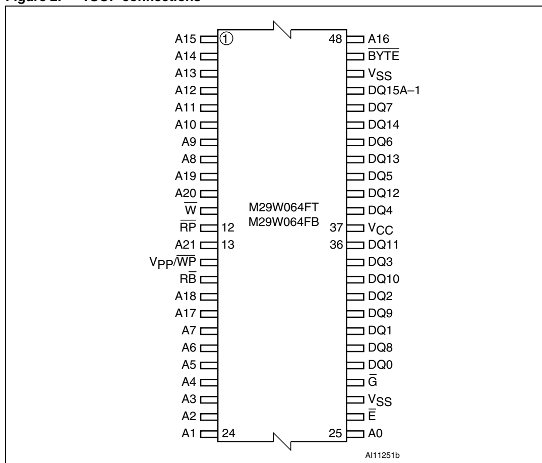
Figure 2. TSOP connections
