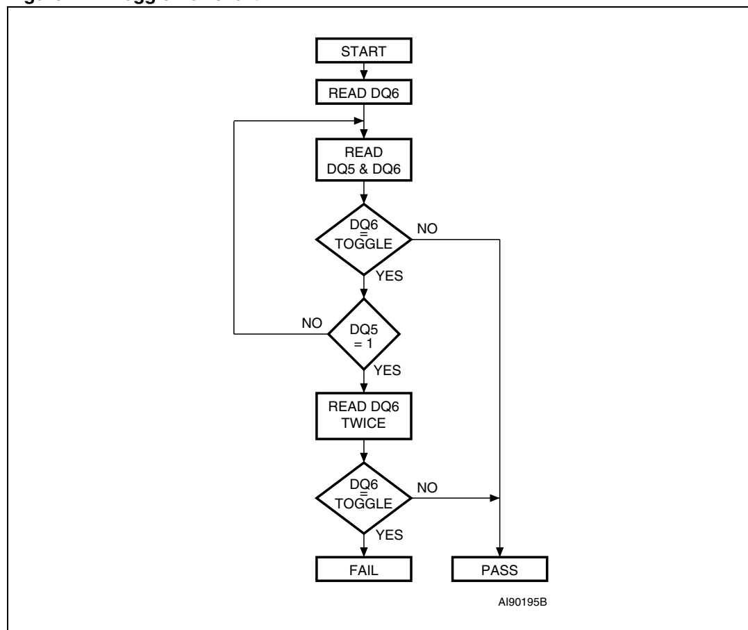
Figure 4. Toggle flowchart
