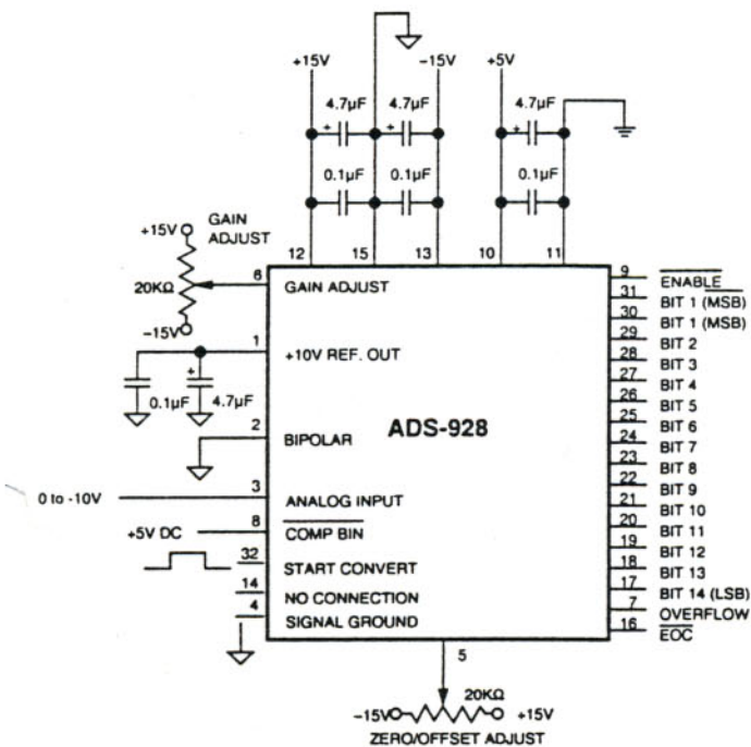
Figure 3. Typical ADS-928 Connection Diagram
