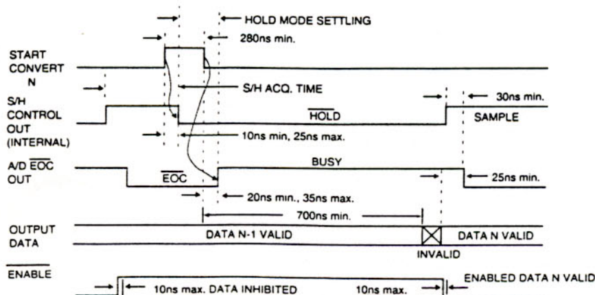
Figure 2. ADS-928 Timing Diagram
