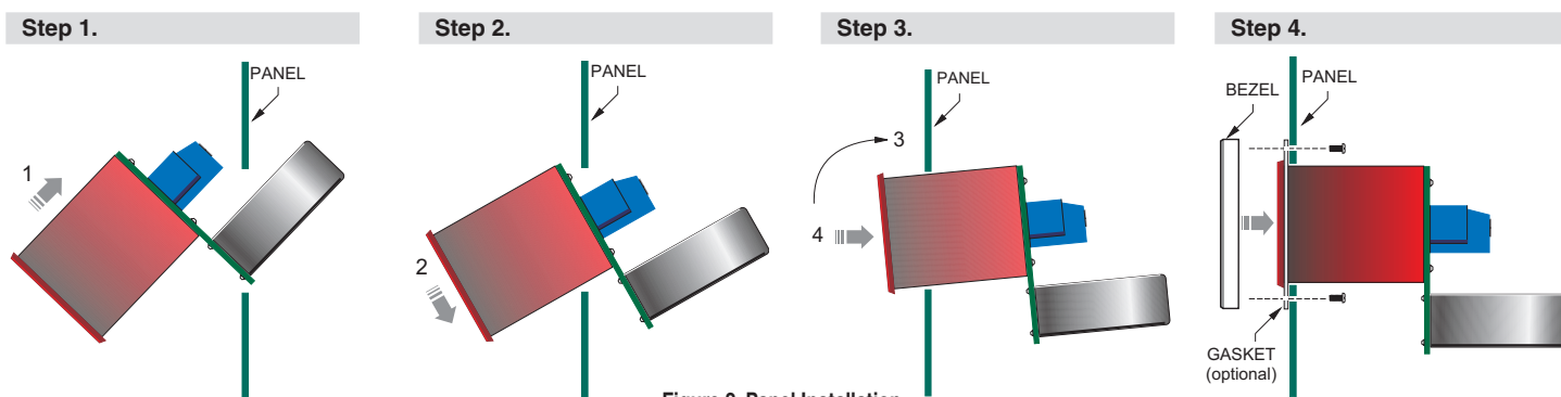
Figure 2. Panel Installation
