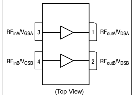
Figure 1. Pin Connections
