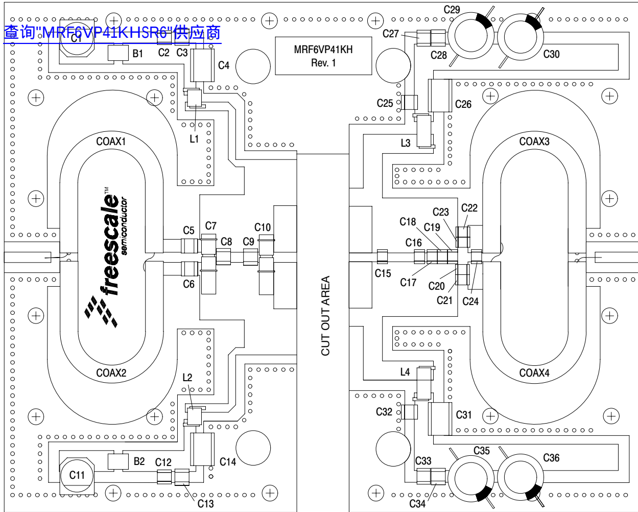
Figure 3. MRF6VP41KHR6 Test Circuit Component Layout
