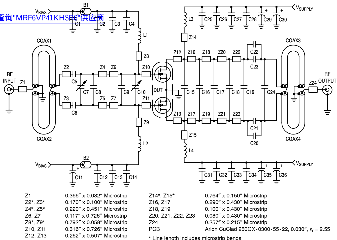
Figure 2. MRF6VP41KHSR6 Test Circuit Schematic
