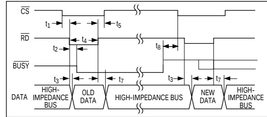
Figure 5. ROM Interface Timing Diagram
