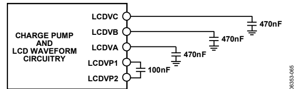
Figure 89. External Circuitry for Charge Pump Option
