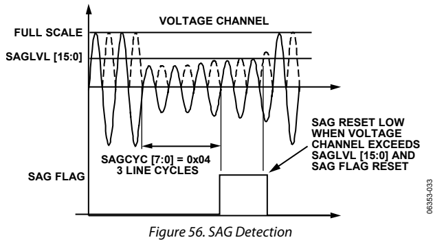
Figure 56. SAG Detection
