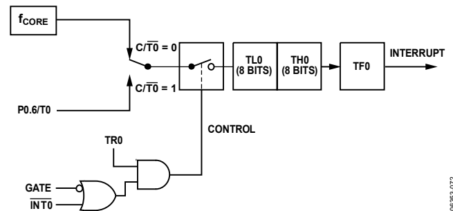
Figure 96. Timer/Counter 0, Mode 1
