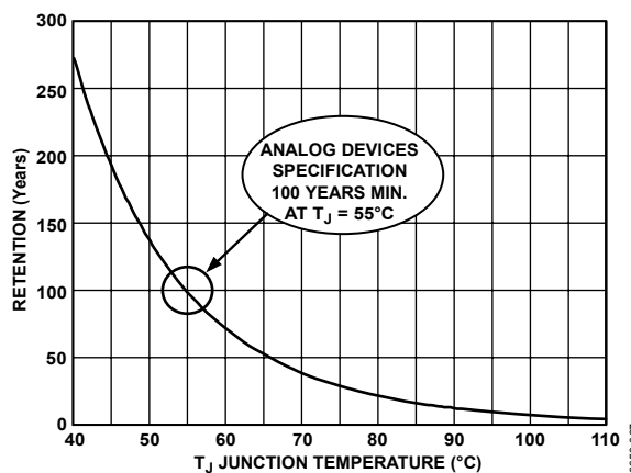
Figure 91. Flash/EE Memory Data Retention
