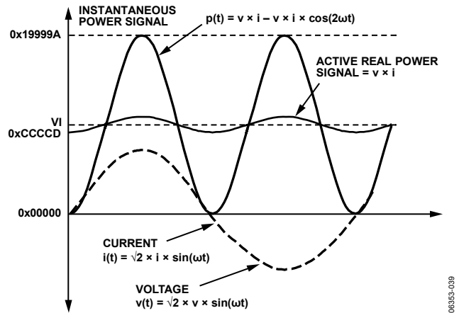
Figure 63. Active Power Calculation
