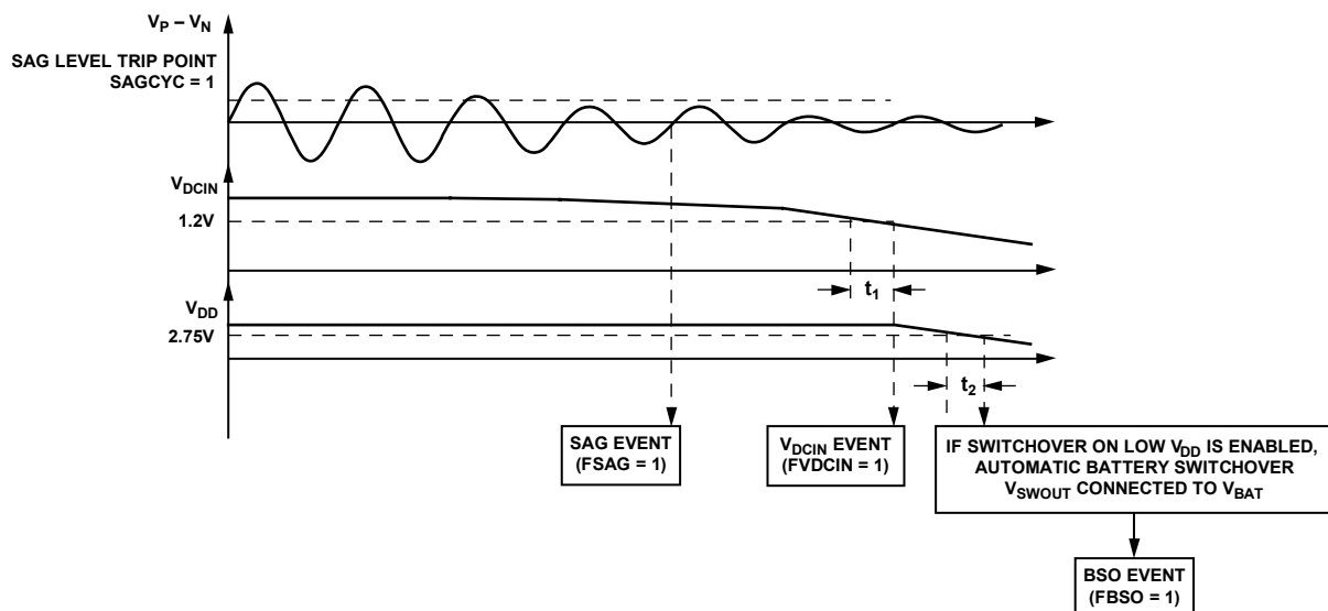
Figure 34. Power Supply Management Interrupts and Battery Switchover with Only V_{DD} Enabled for Battery Switchover
