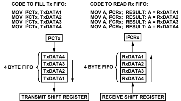
Figure 113. I 2 C FIFO Operation
