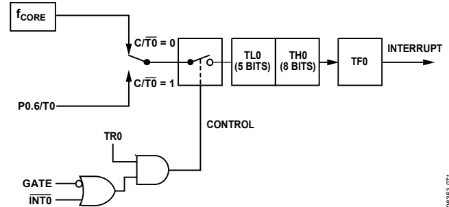
Figure 95. Timer/Counter 0, Mode 0
