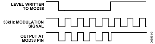
Figure 115. 38 kHz Modulation
