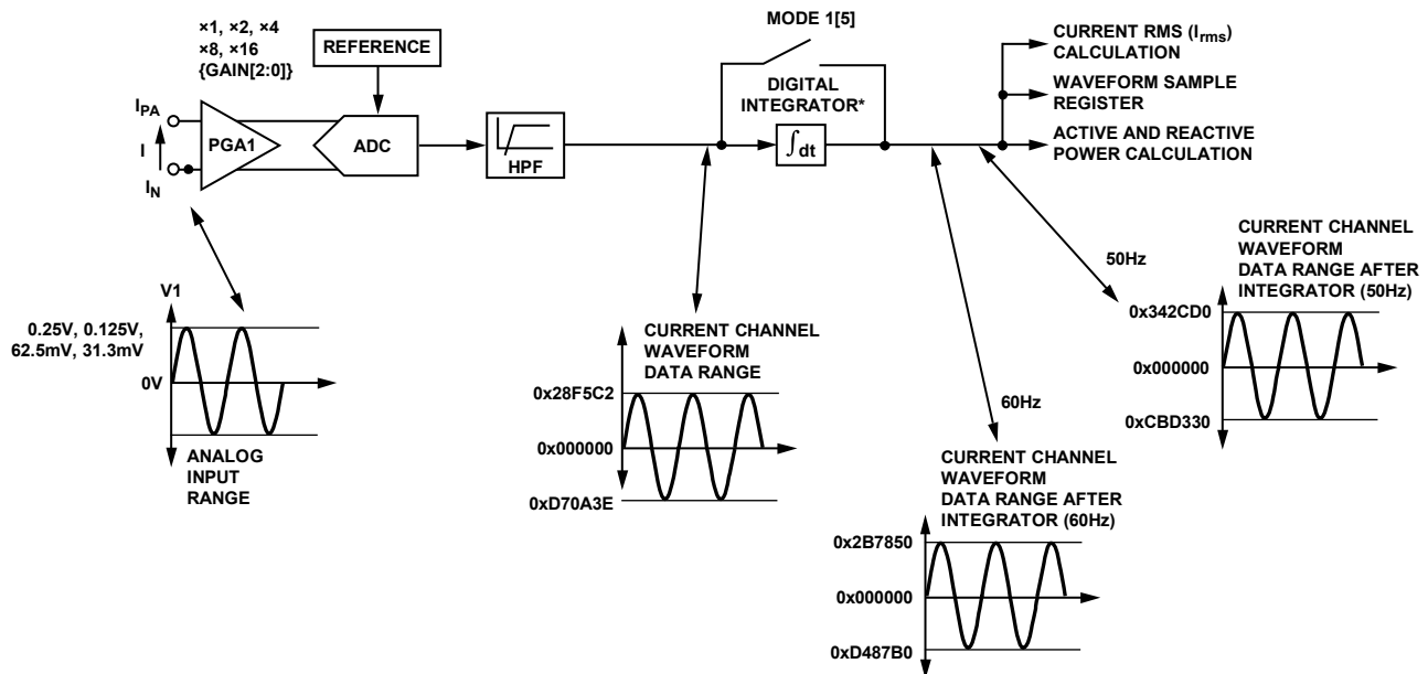
Figure 45. ADC and Signal Processing in Current Channel with \text{PGA1} = 1, 2, 4, 8, \text{ or } 16 for ADE7566 and ADE7569
