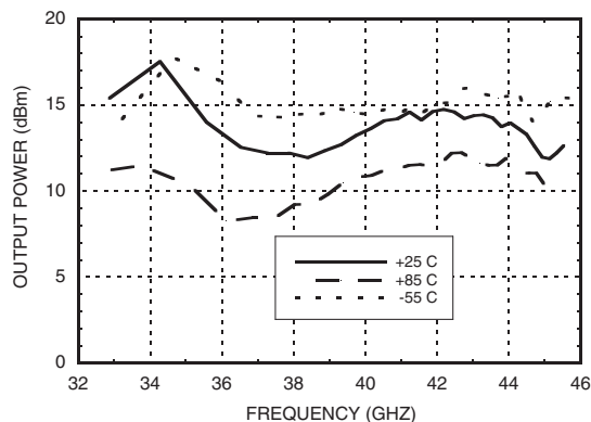
Output Power vs. Frequency, V_{cc} = +5V
