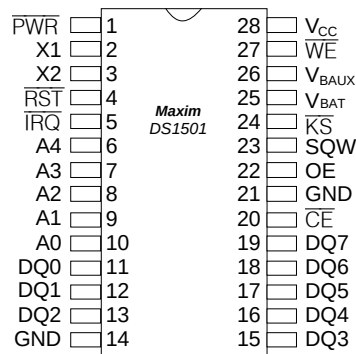
DIP, SO
