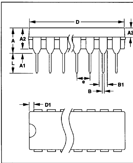
Plastic DIP PLASTIC DUAL-IN-LINE PACKAGE (0.300 in.)
