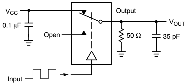
Figure 2. t_{ON} / t_{OFF} V_{is} = V_{CC}
