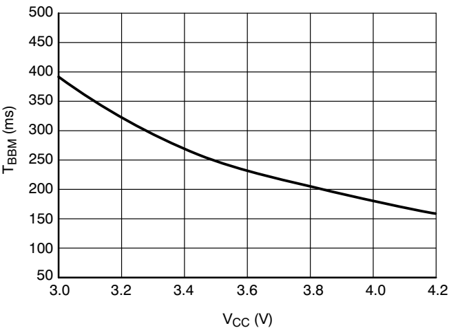
Figure 14. NLA6233 T BBM vs. V CC
