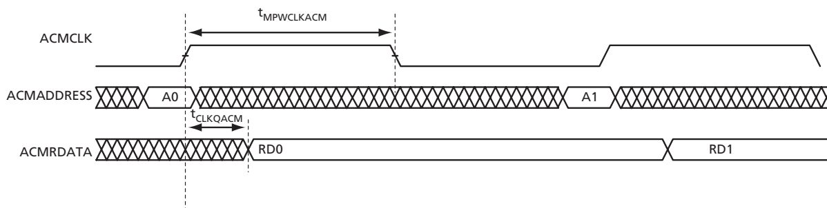
Figure 2-90 • ACM Read Waveform
