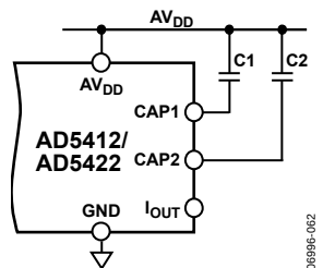
Figure 69. I_{OUT} Filtering Capacitors
