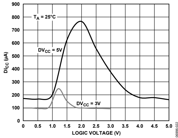
Figure 7. D_{Le} vs. Logic Input Voltage
