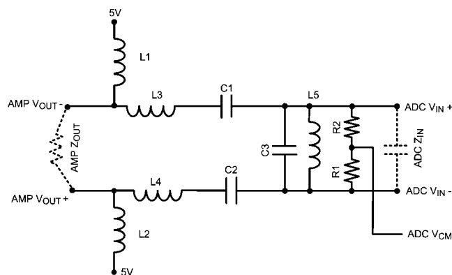
FIGURE 7. Sample Filter
