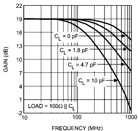
Frequency Response with Capacitive Load
