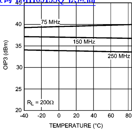
OIP3 Over Temperature 查询"LMH6515SQ"供应商
