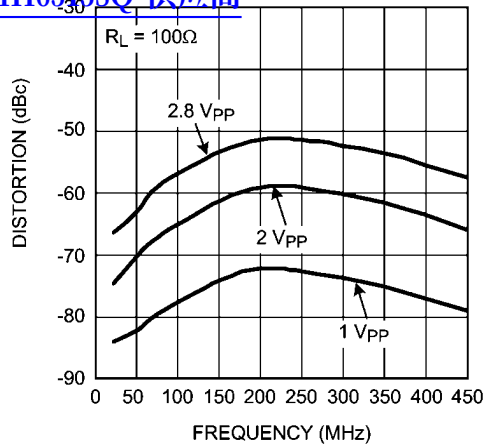
HD3 vs. Frequency 查询"LMH6515SQ"供应商
