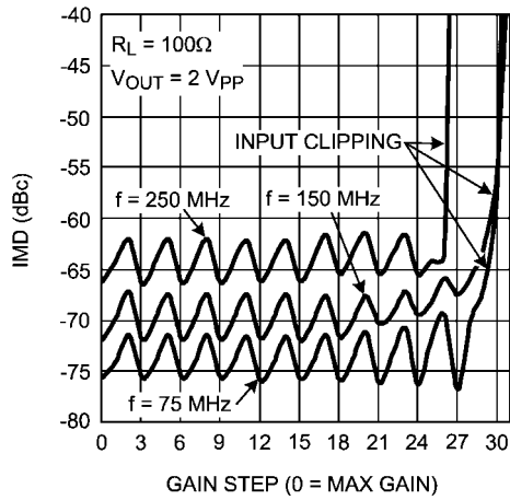
IMD3 Low Gain Mode
