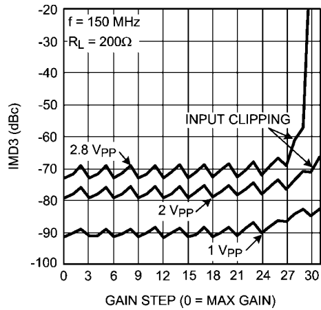
IMD3 High Gain Mode
