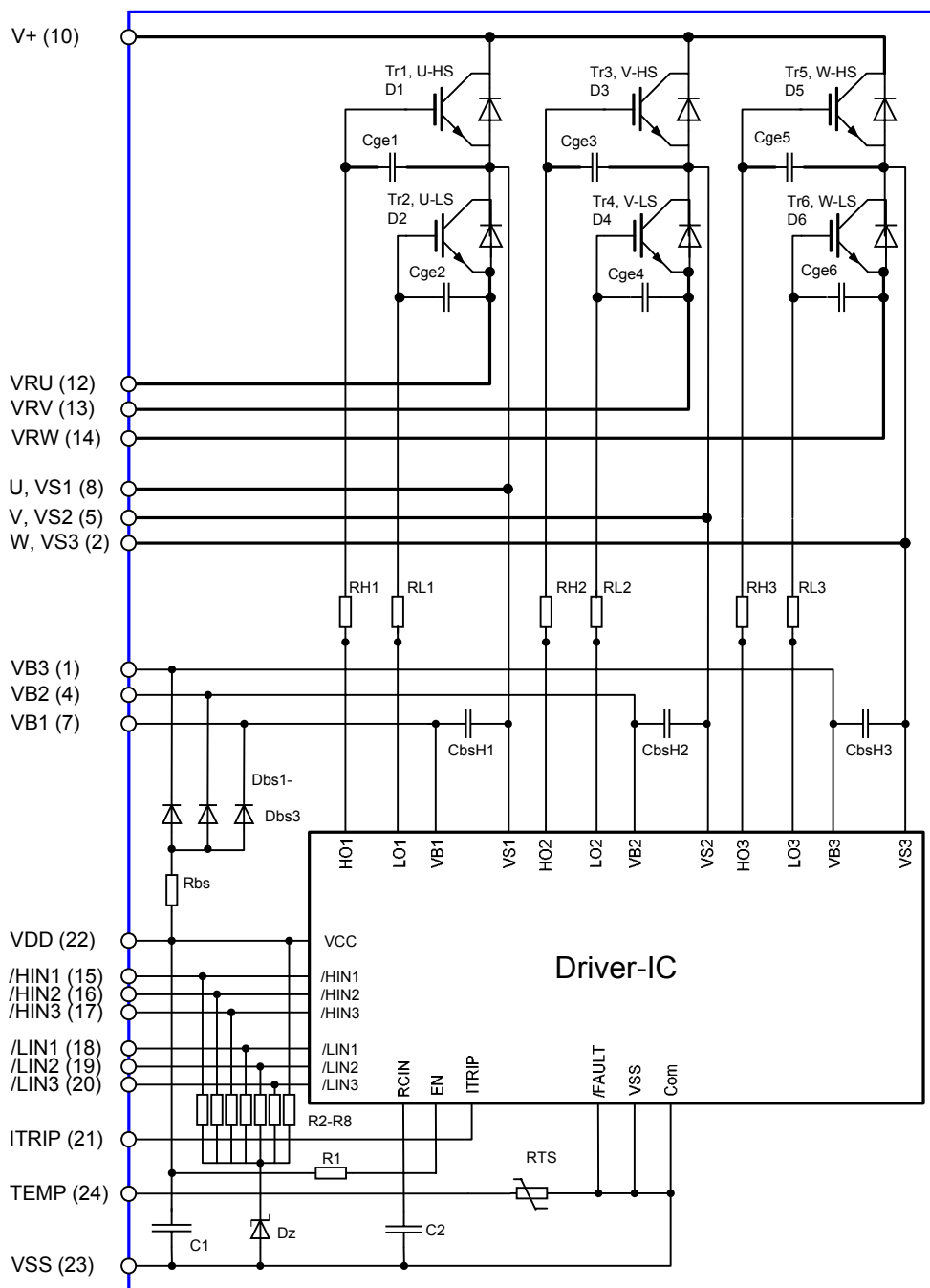
Figure 1: Internal Schematic
