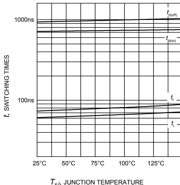
Figure 8. Typical switching times as a function of junction temperature (inductive load, V_{CE} = 300\text{V} , I_C = 15\text{A} , Dynamic test circuit in Figure A)
