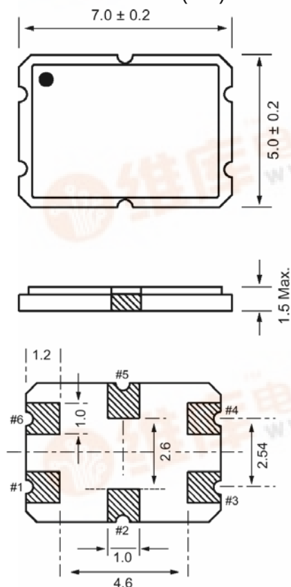
Figure 1) Top, Side and Bottom Views
