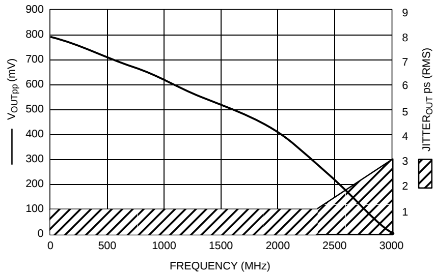
Figure 5. F_{max}/Jitter for \overline{Q} Output
