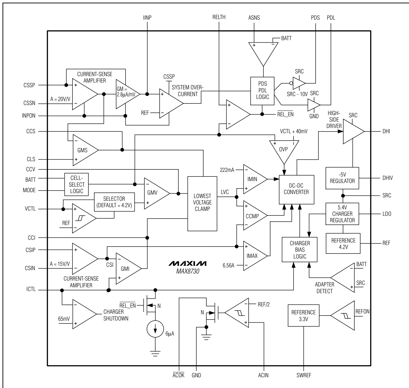
Figure 2. Functional Diagram
