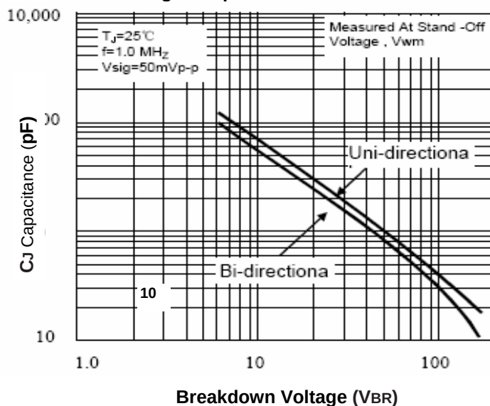
Fig.6- Capacitance
