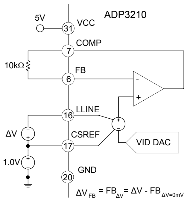
Figure 4. Positioning Accuracy
