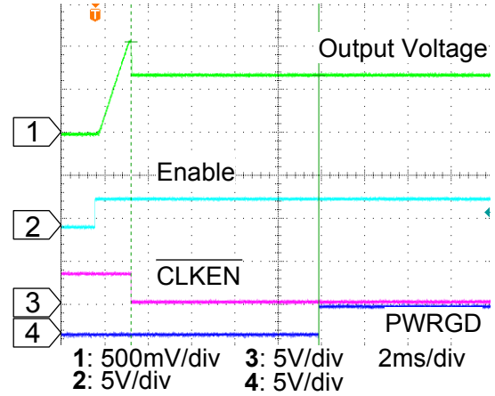
Figure 9. Start-UP Waveforms
