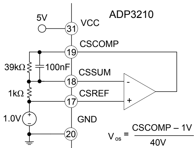
Figure 3. Current-Sense Amplifier V_{os}
