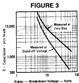
Typical Capacitance vs. Breakdown Voltage (Unidirectional Types)
