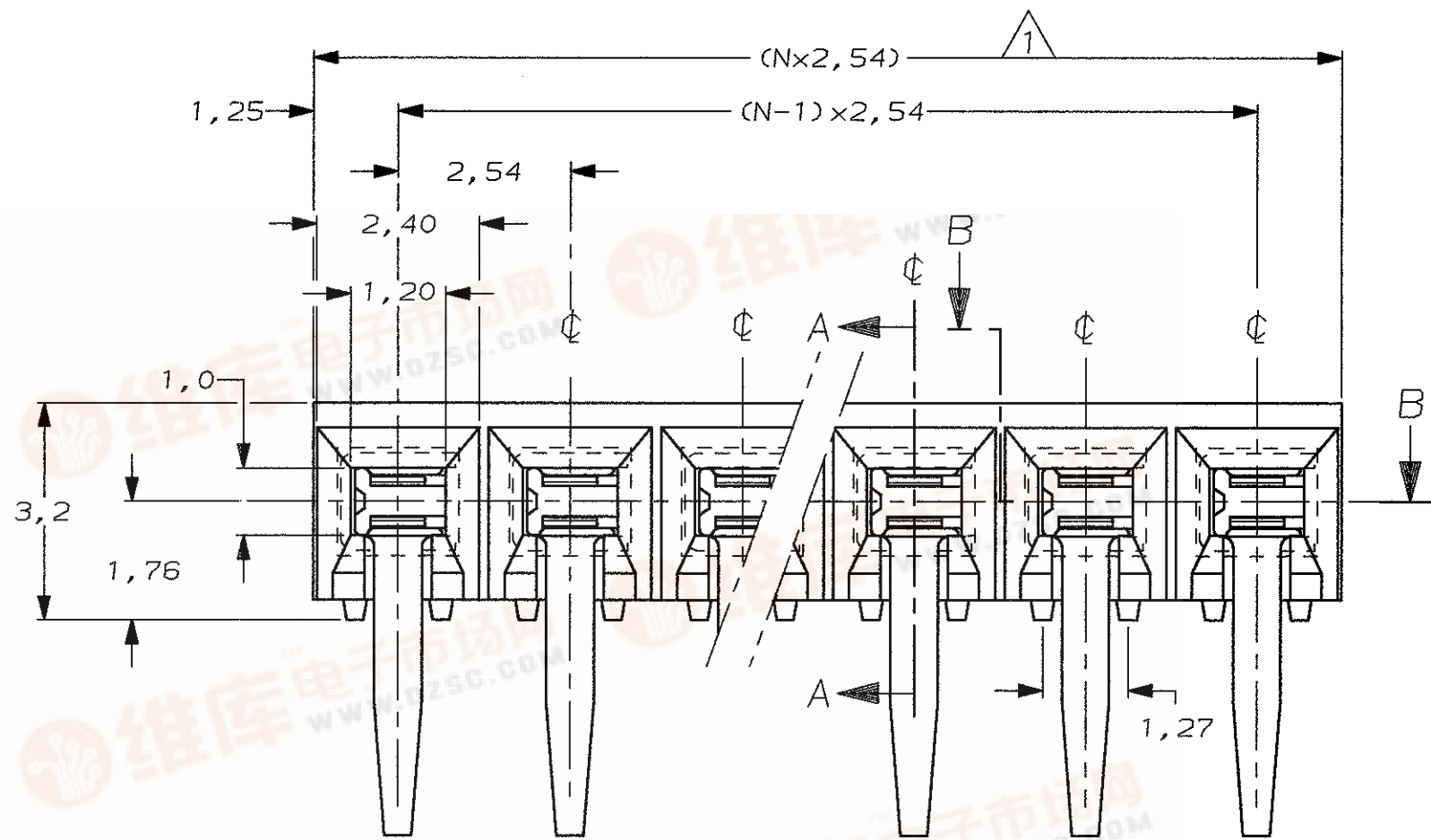
FRONT VIEW
