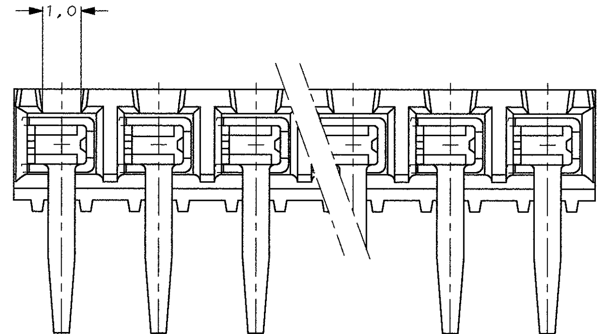
REAR VIEW
