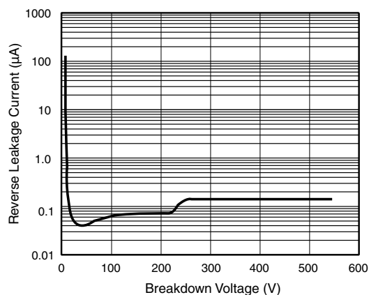
Figure 13. Typical Reverse Leakage Characteristics
