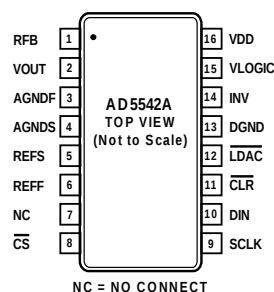
Figure 12. AD5542A 16-Lead TSSOP Pin Configuration
