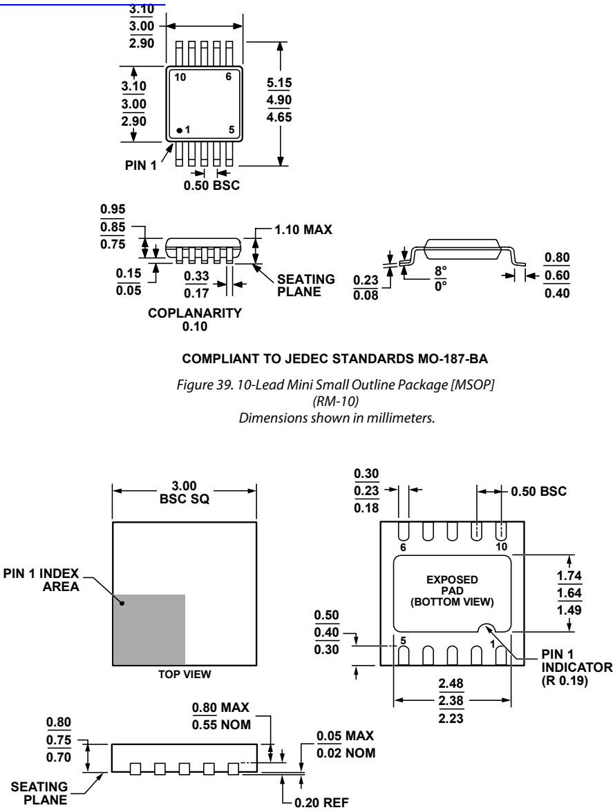
Figure 40. 10-Lead Lead Frame Chip Scale Package [LFCSP] (CP-10-9) Dimensions shown in millimeters.
