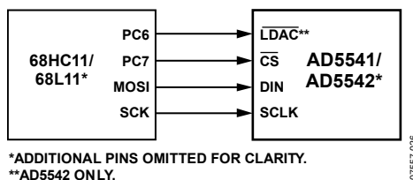
Figure 34. AD5541/AD5542 to 68HC11/68L11 Interface
