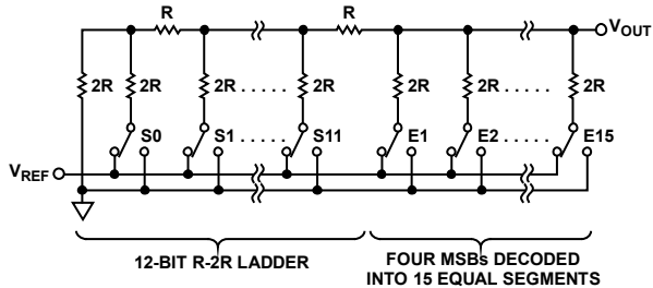
Figure 30. DAC Architecture
