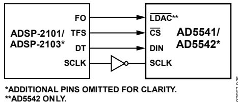
Figure 33. AD5541/AD5542 to ADSP-2101/ADSP-2103 Interface
