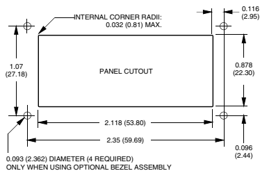
RECOMMENDED DRILL AND PANEL CUTOUT DIMENSIONS
