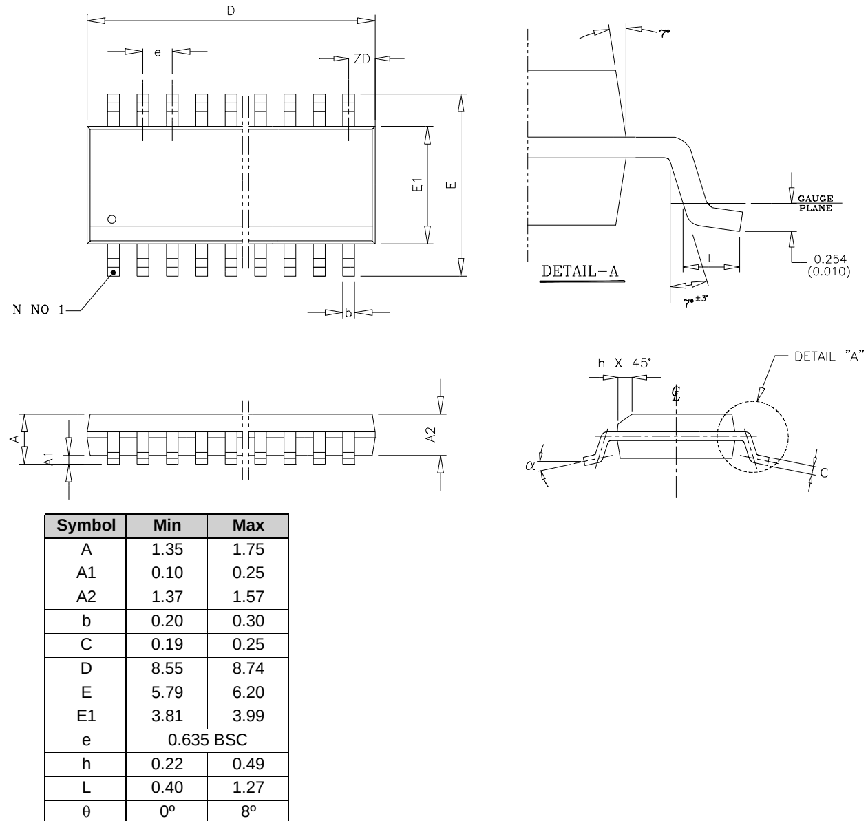
Figure 21. QSOP-24 Package
