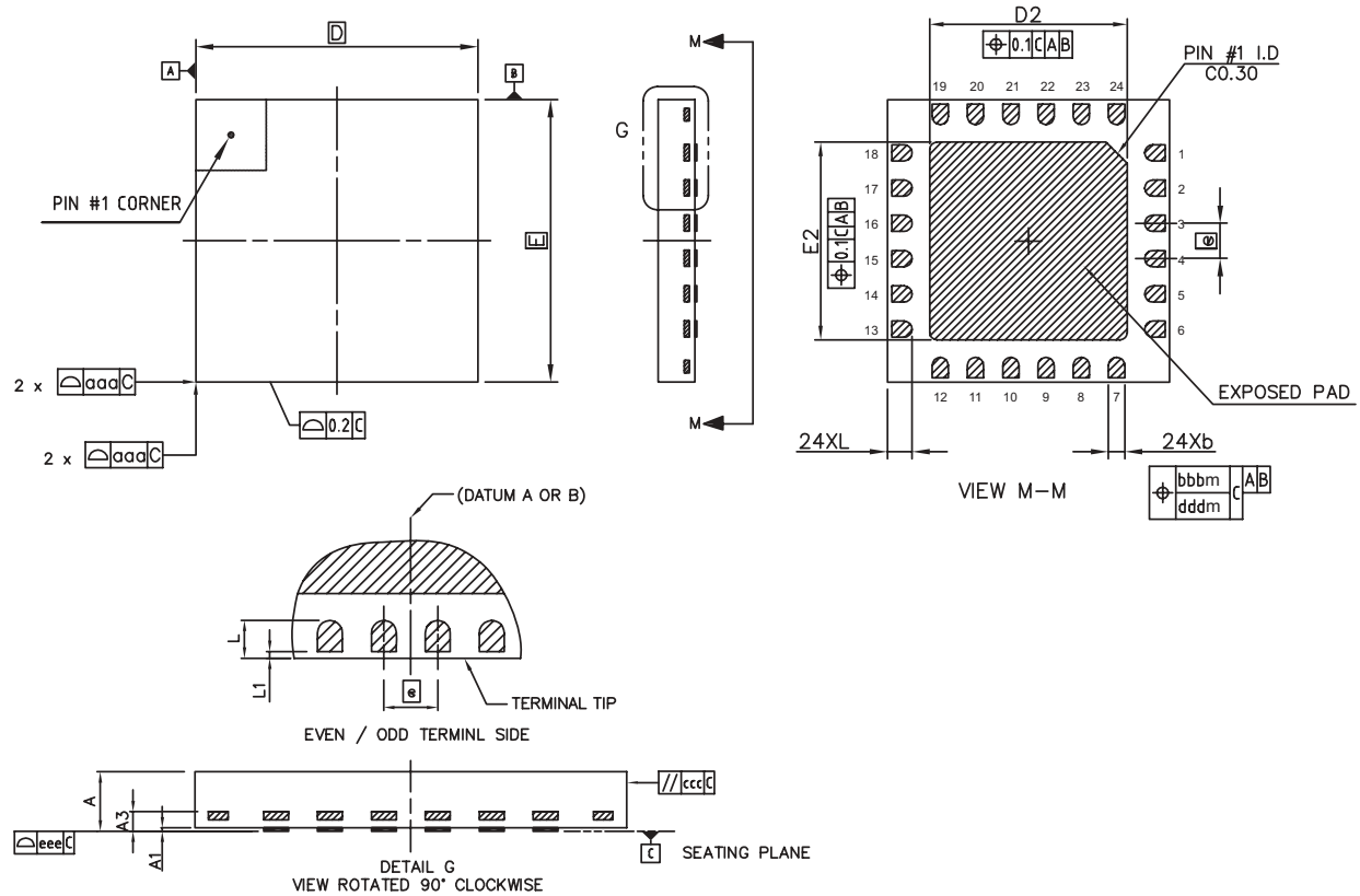
Figure 22. TQFN(4x4)-24 Package
